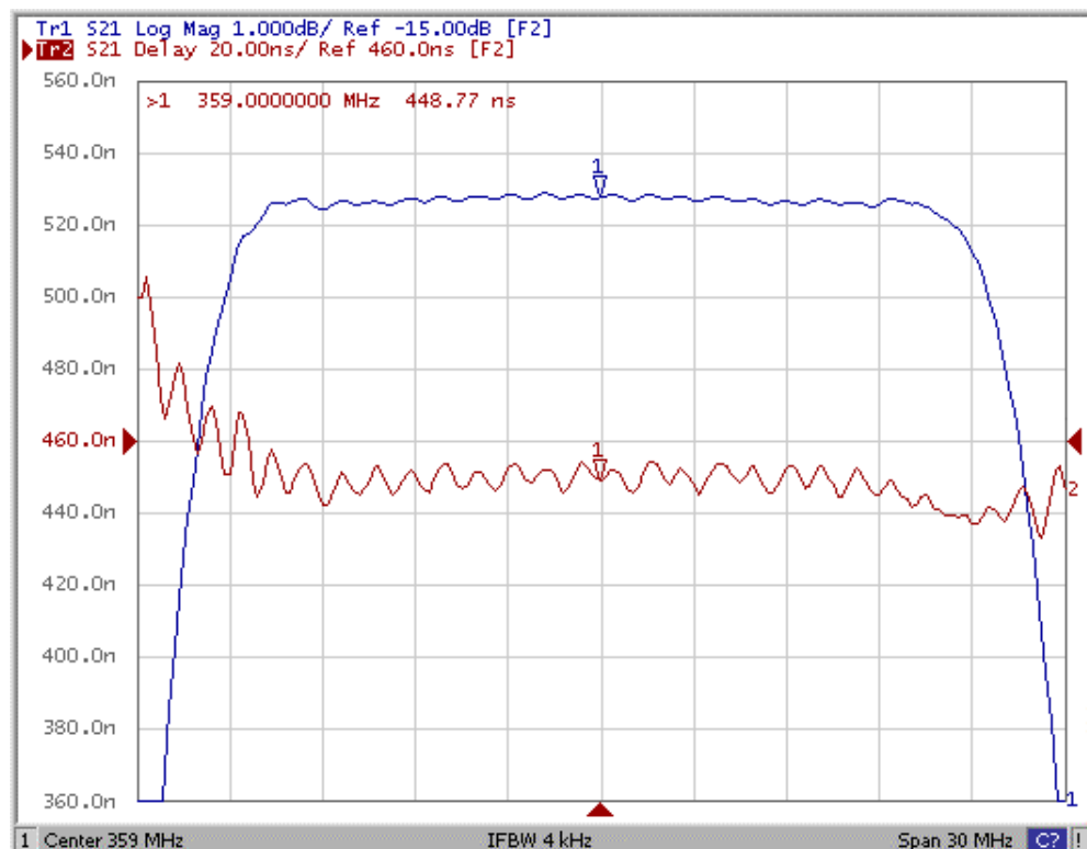
Fig2. Horizontal: 3.0MHz/Div Vertical: 20nec/Div
