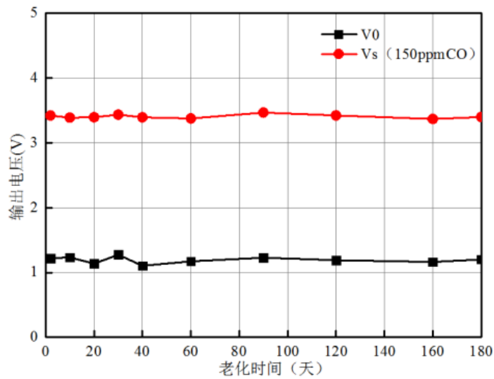
Fig7.long-term Stability
