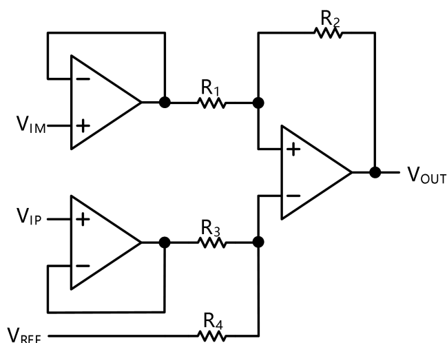
Figure 6. Instrument Amplifier
