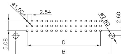
RECOMMEND PCB LAYOUT(FOR FEMALE) TOLERANCE=±0.05mm
