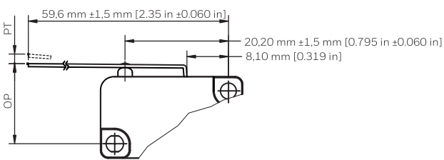
FIGURE 13. V19 SERIES A03/LONG STRAIGHT LEVER
