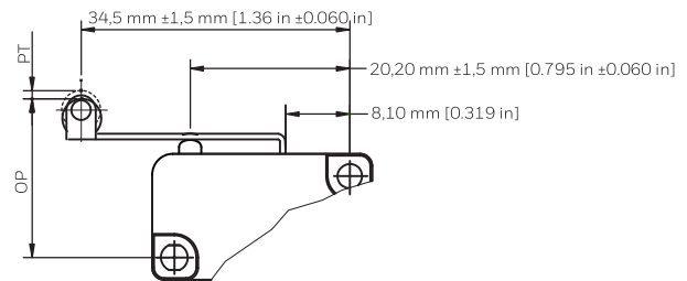
FIGURE 16. V19 SERIES A06/ROLLER LEVER
