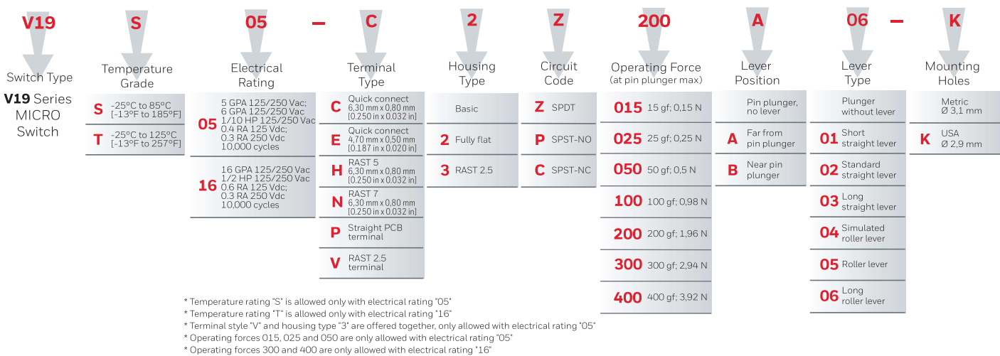
FIGURE 1. PRODUCT NOMENCLATURE
