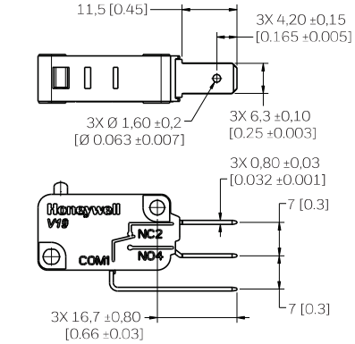
FIGURE 9. V19 SERIES N-STYLE RAST-7 250# CONNECTOR
