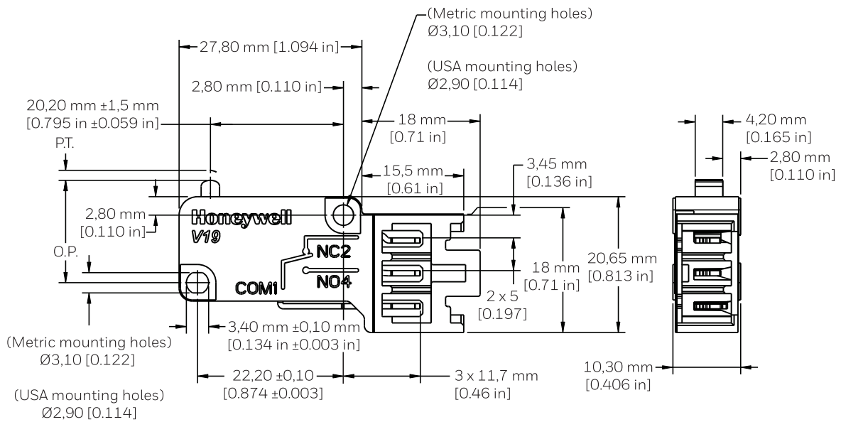
FIGURE 5. V19 SERIES RAST 2.5 SWITCH DIMENSIONS
