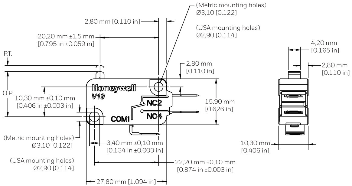
FIGURE 3. V19 SERIES STANDARD SWITCH DIMENSIONS
