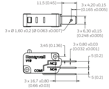
FIGURE 7. V19 SERIES H-STYLE RAST-5 250# CONNECTOR
