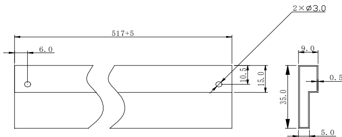
图 9 内包装塑料条管 Figure 9 Internally plastic tube
